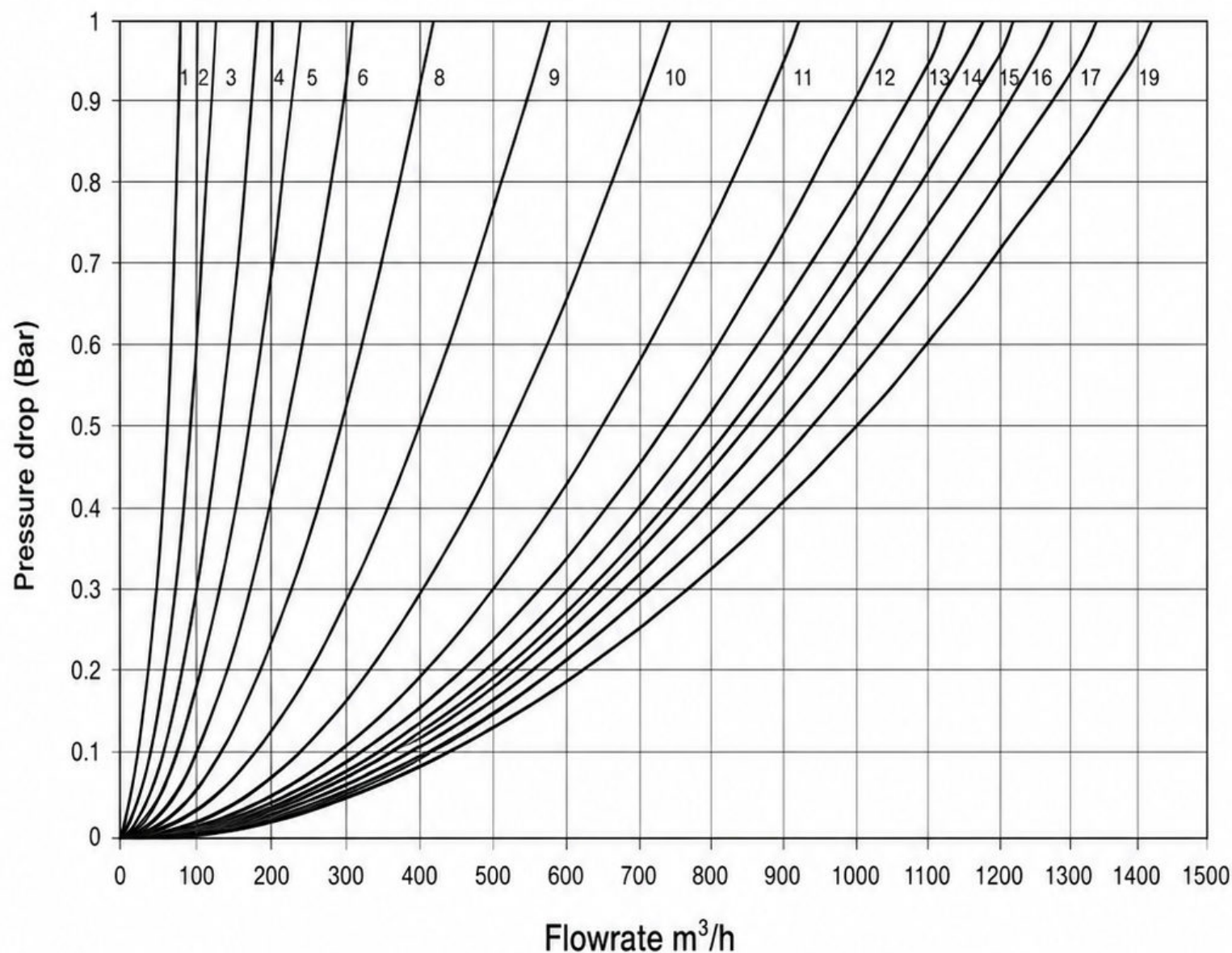
FLOW DIAGRAM
